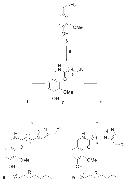
Scheme 2. Reagents and conditions: a) 8-azidooctanoic acid, Et 3 N, PPAA, 53%; b) 1-decyne, tert -butanol/water, CuSO 4 ·5 H 2 O, sodium ascorbate, 50%; c) 1-decyne, [Cp*Ru(PPh 3 ) 2 Cl], benzene, 6%. PPAA = propanephosphonic acid anhydride.
